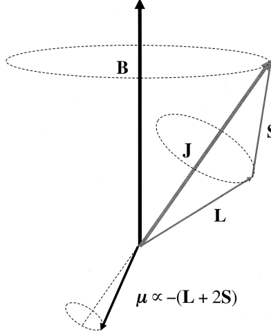
Figure 14: Precession about an external magnetic field of total angular momentum \mathbf{J} and total magnetic moment \boldsymbol{\mu} for the case of a weak magnetic field.
