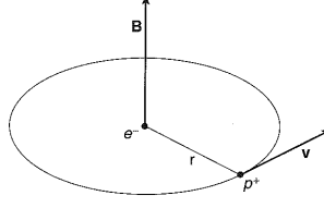
Figure 9: Proton rotating around electron. (Taken from McIntyre pg. 389)
