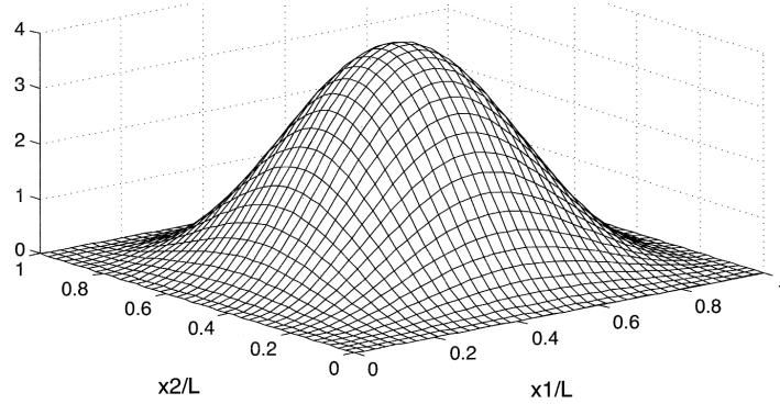
Figure 17: Probability density distribution for the ground state
