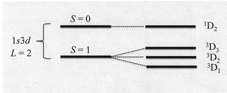
Figure 22: The energy levels of helium corresponding to the excited electron configuration 1s3d .
