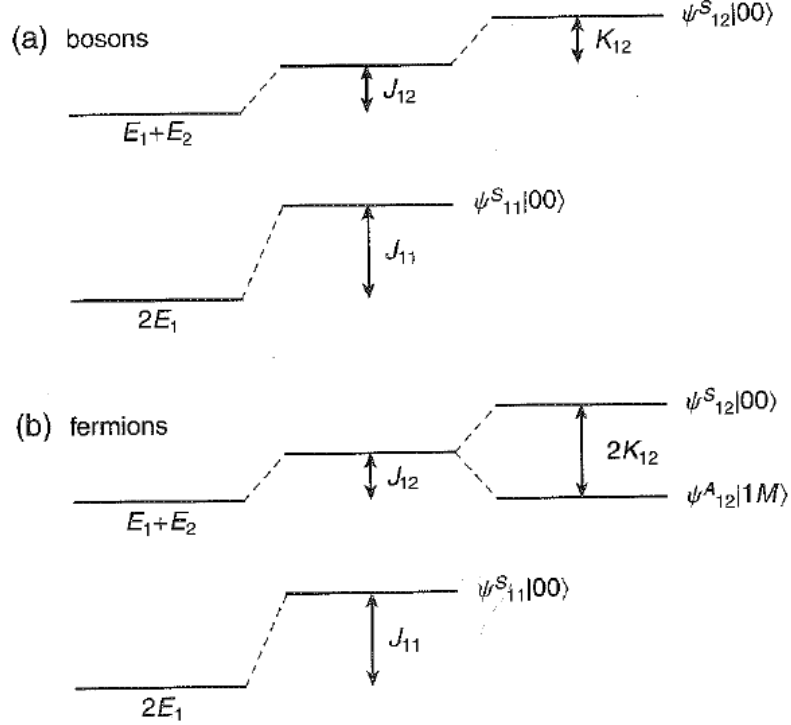
Figure 19: Energies and state vectors for the ground and first excited states of two identical particles (taken from McIntyre Sec. 13.3 pg 426)
