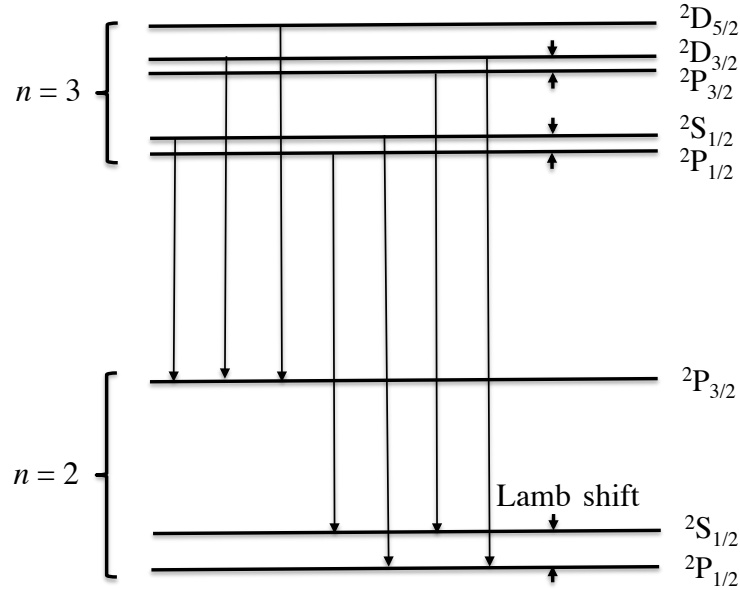
Figure 11: Fine structure of the n = 2, 3 hydrogen levels. The spacing between the fine structure levels is greatly exaggerated compared to the spacing between principal levels. The allowed transitions between n = 3 and n = 2 , i.e. the fine structure H_\alpha line, are also shown
