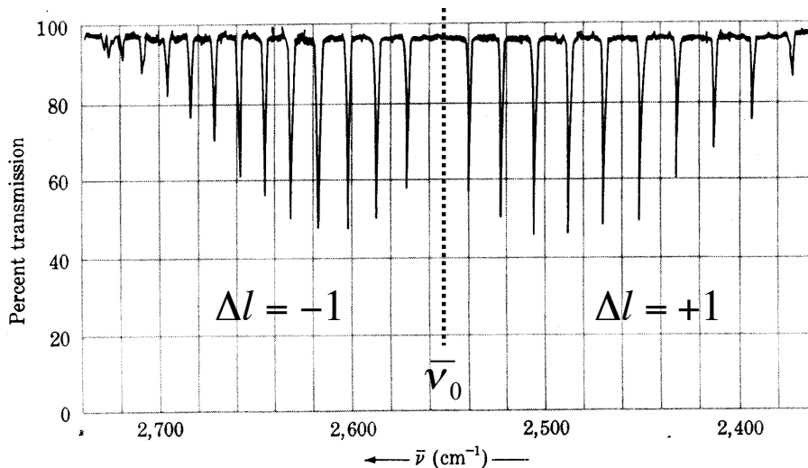
Figure 5: The vibrational-rotational absorption spectrum for HBr. (based on Figure 8-5, Basic Principles of Spectroscopy , R. Chang, McGraw-Hill, New York, 1971)
