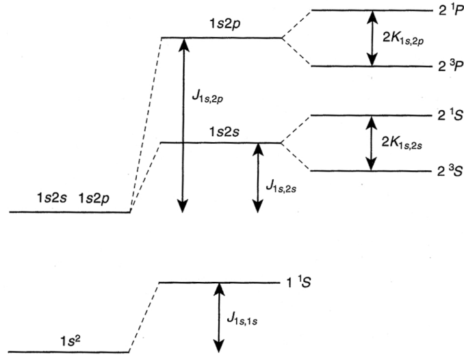
Figure 20: The effect of the electron-electron interaction and the exchange interaction on helium energy levels. Reproduced from Figure 13.9, McIntyre p432.
