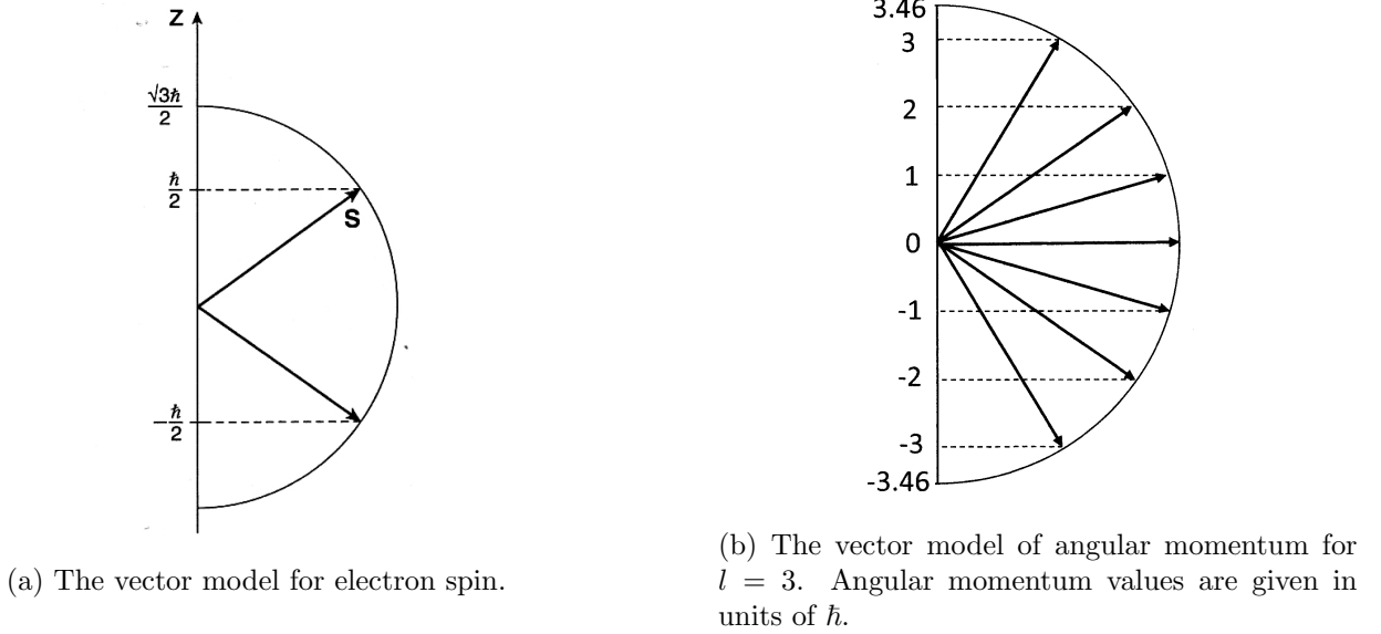
Figure 4: The vector model
