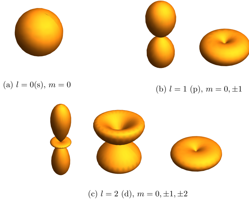
Figure 6: Spherical Harmonics
