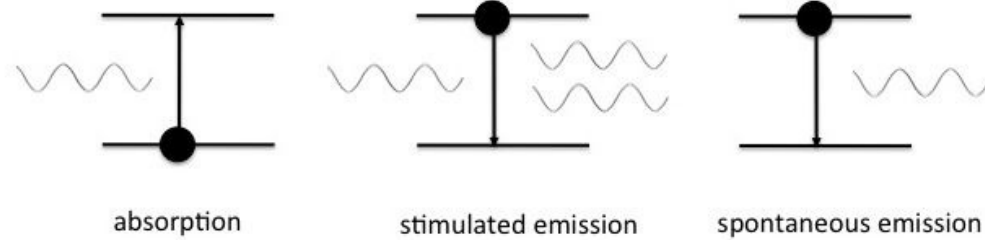
Figure 8: (a) absorption; (b) stimulated emission; (c) spontaneous emission
