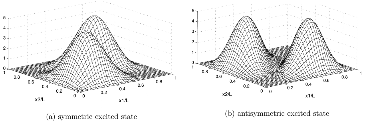
Figure 18: Probability density distributions
