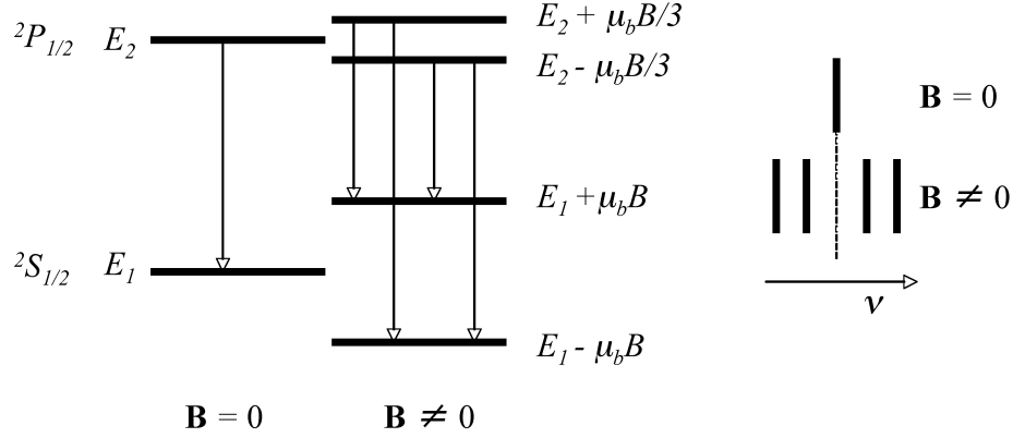
Figure 15: The Zeeman splitting of the ^2S_{1/2} and ^2P_{1/2} levels of an alkali atom. Also shown are the four allowed transitions,
