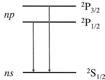
Figure 21: The energy levels of the sodium corresponding to the ground and first excited electron configurations. The two allowed transitions shown are the well-known yellow doublet of sodium: \lambda = 589.0 and 589.6 nm
