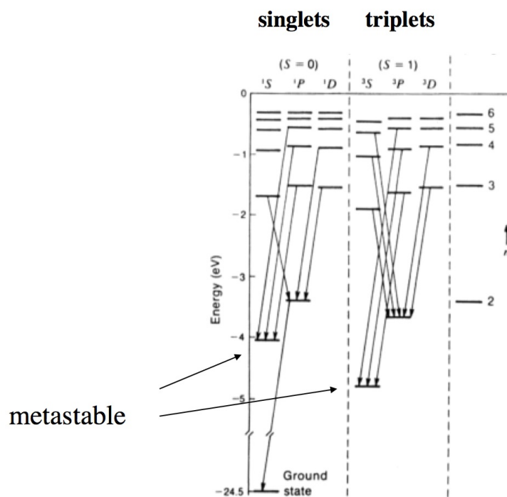
Figure 23: Energy levels and allowed transitions for helium. Singlet and triplet states are shown separately. Note that the lowest singlet and triplet states are metastable. Based on Figure 13-5, An Introduction to Quantum Mechanics , A.P. French & E.F. Taylor (Thomas Nelson 1979).
