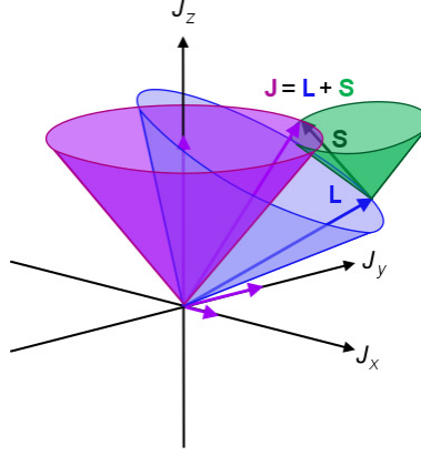
Figure 10: LS coupling (taken from Wikipedia)
