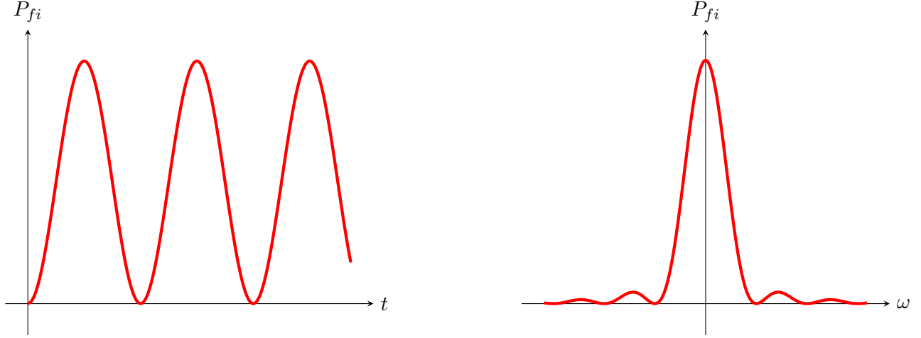
Figure 24: Probability as a function of time (left-hand side) and frequency (right-hand side)
