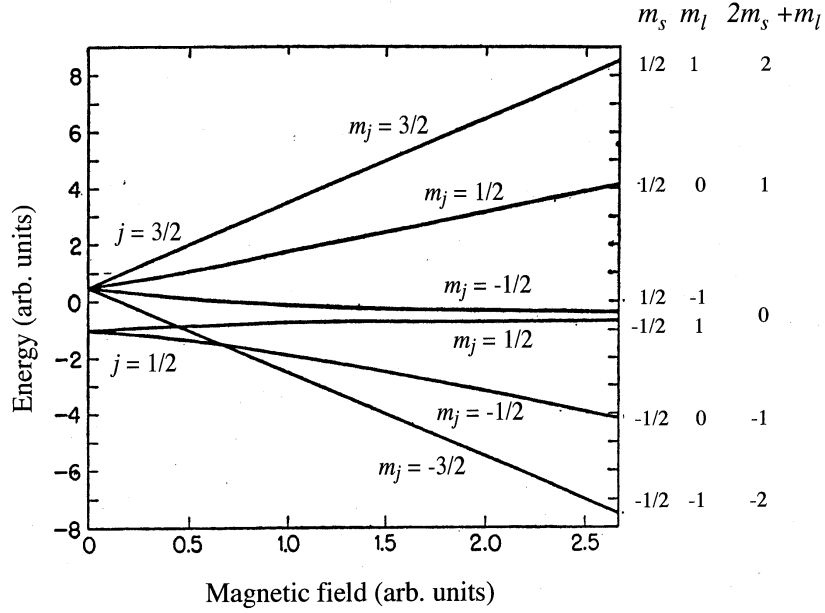
Figure 16: The energy levels of the np first excited state of the optical electron of an alkali atom as a function of magnetic field. The two levels have spectroscopic notations ^2P_{3/2} and ^2P_{1/2} . (based on Figure 93, Introduction to Modern Physics , F.K. Richtmeyer, E.H. Kennard and T. Lauritsen (McGraw-Hill, New York, 1955))
