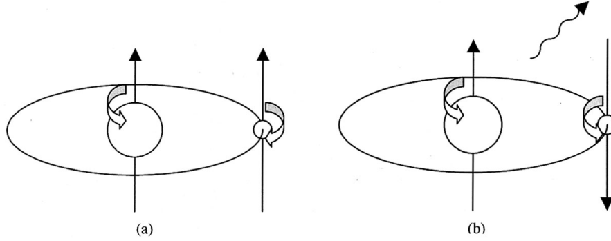
Figure 12: The ‘spin-flip’ transition between the hyperfine levels of the hydrogen ground state that leads to emission at 21 cm (1420 Hz).
