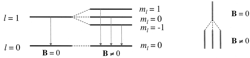
Figure 13: The effect of a weak external magnetic field on singlet states with l = 1 and l = 0 . The splitting of the allowed transition between the levels is also shown on the right.
